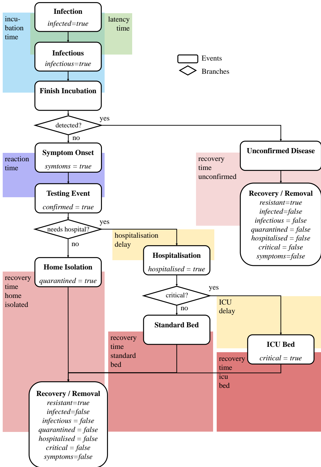
Figure 2: State chart of the patient pathway of a person-agent in the agent-based COVID-19 model. Only those state variables that are changed by the corresponding event are labelled, all others remain at the current value. The initial state of all infection-specific state variables is false .
